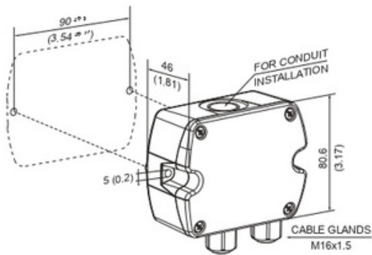
Type T13 (outdoor)
