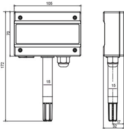
Dimensions Wall version Type W
