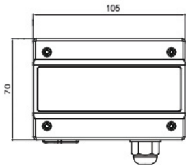
Duct version Type D / Probe length 100 mm
